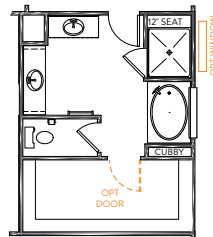
LUXURY BATH OPT 3 42" X 60" GARDEN TUB w/CERAMIC TUB SURROUND 42" X 48" FRAMED TILE SHOWER BASE TILE WALLS w/12" TILE SEAT
